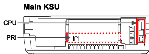
Figure 1-9 Digital Trunk Clocking Example 3
