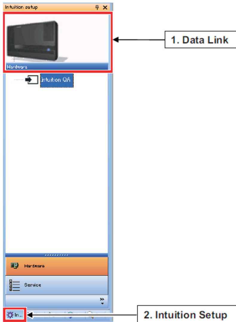
Figure 1-30 Navigation Bar
