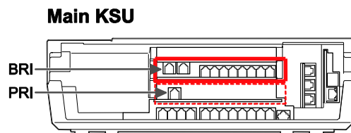
Figure 1-8 Digital Trunk Clocking Example 2
