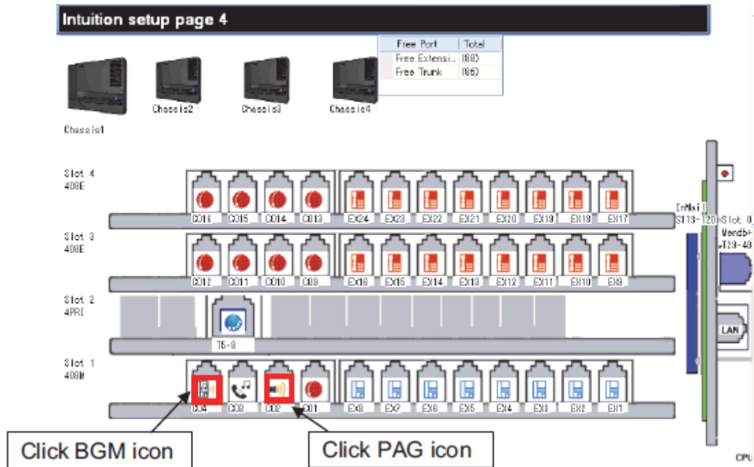
Figure 1-38 KSU View
